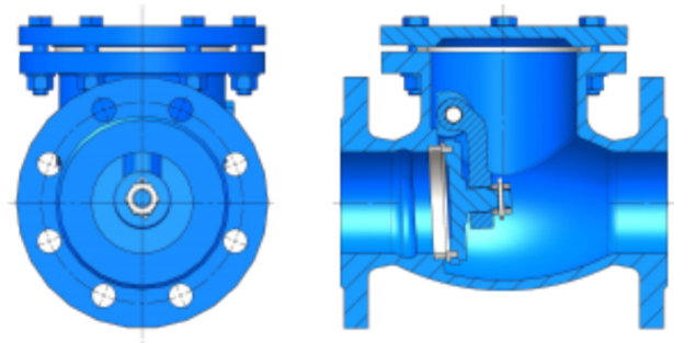
Check valve Swing type
