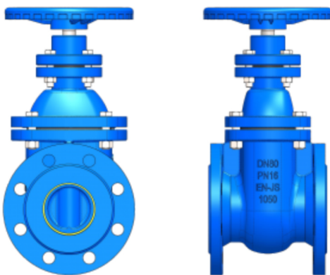
Gate valve
